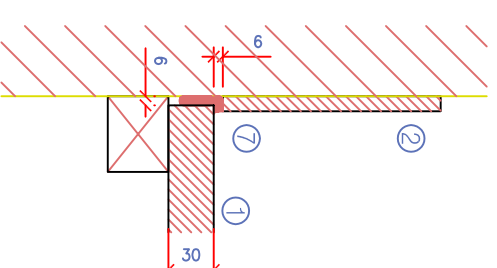
worktop/mastic seal detail scale 1:5
