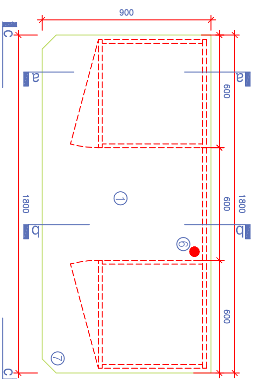
plan (scale 1:20)
