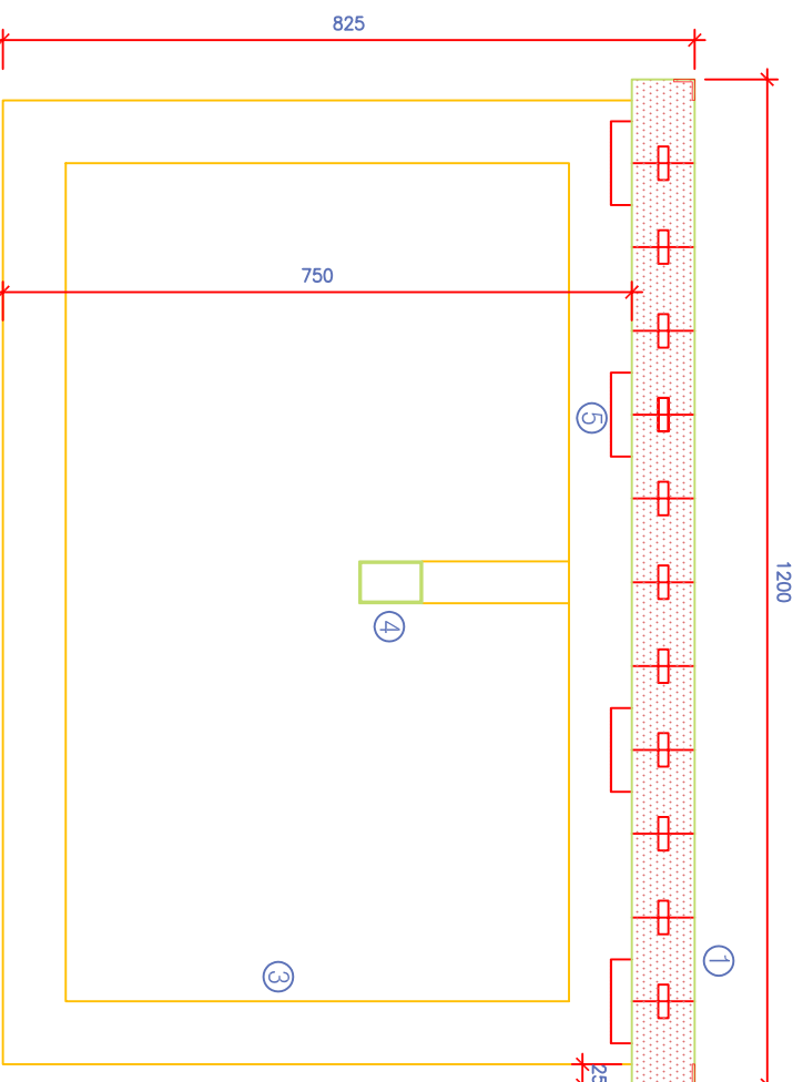
section a-a (1:10)
