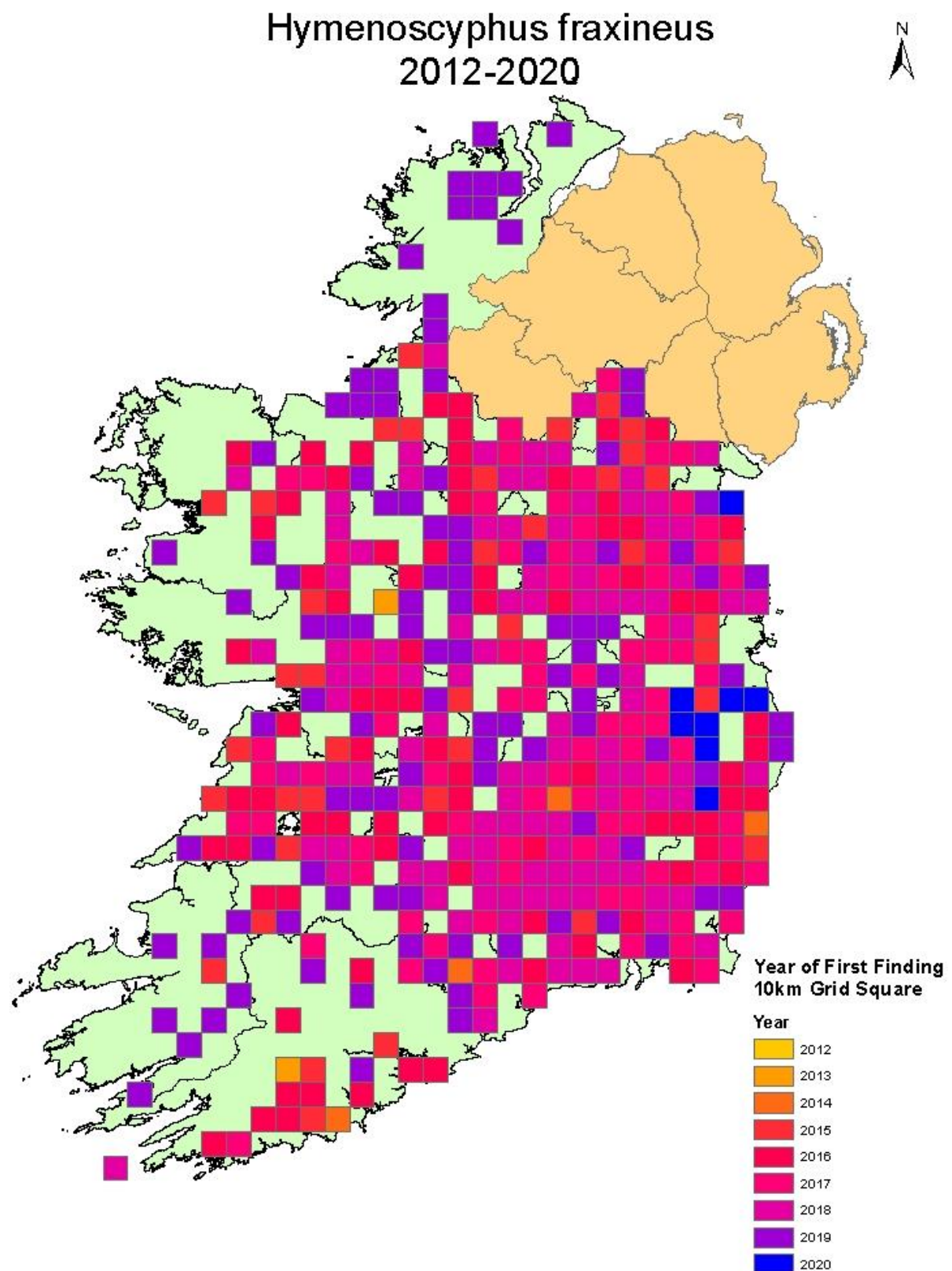
Figure 33. Ash Dieback findings in Ireland 2012 – 2020.
