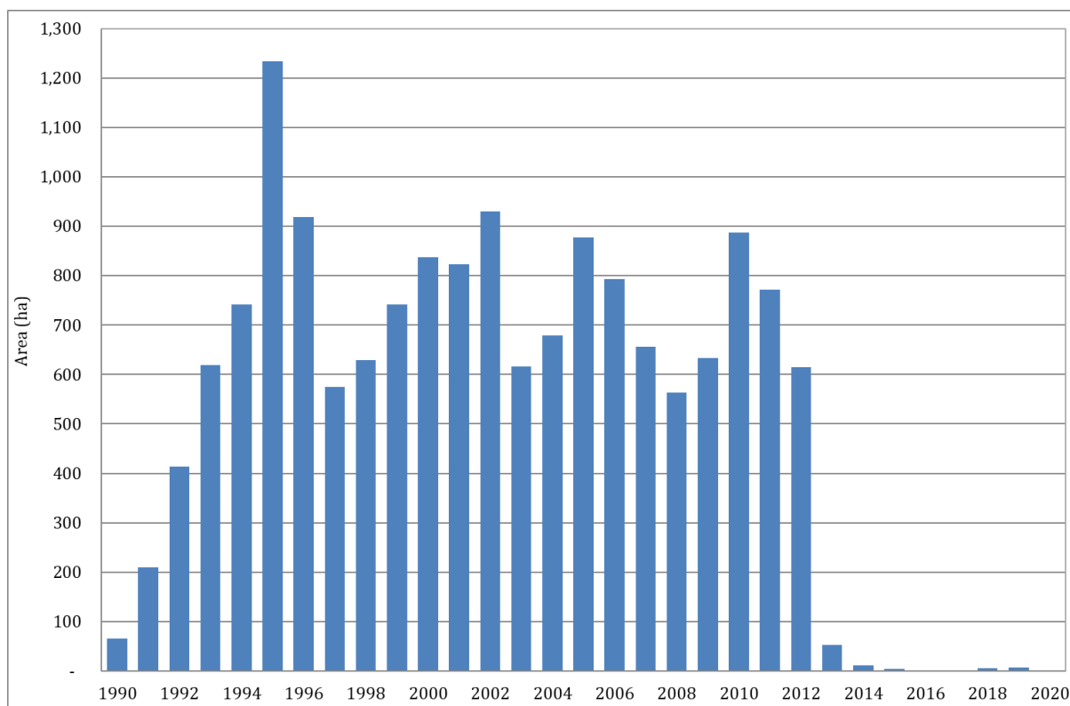
Figure 9. Extent of ash afforestation (1990-2020).
