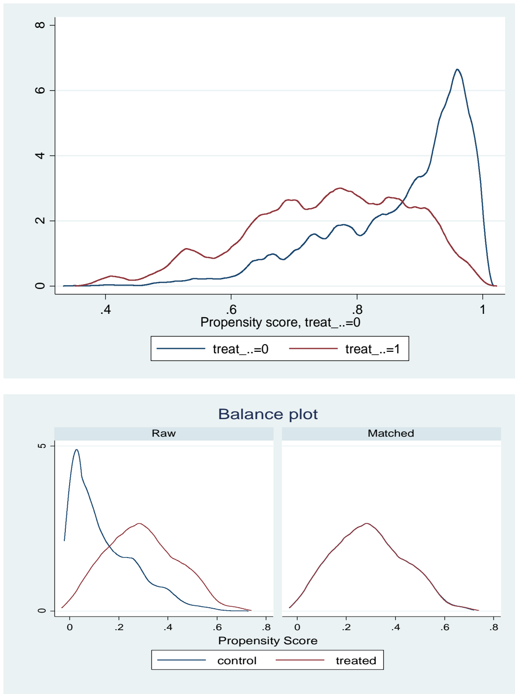
Figure 4.1: Illustration of Validity of Overlap Assumption
