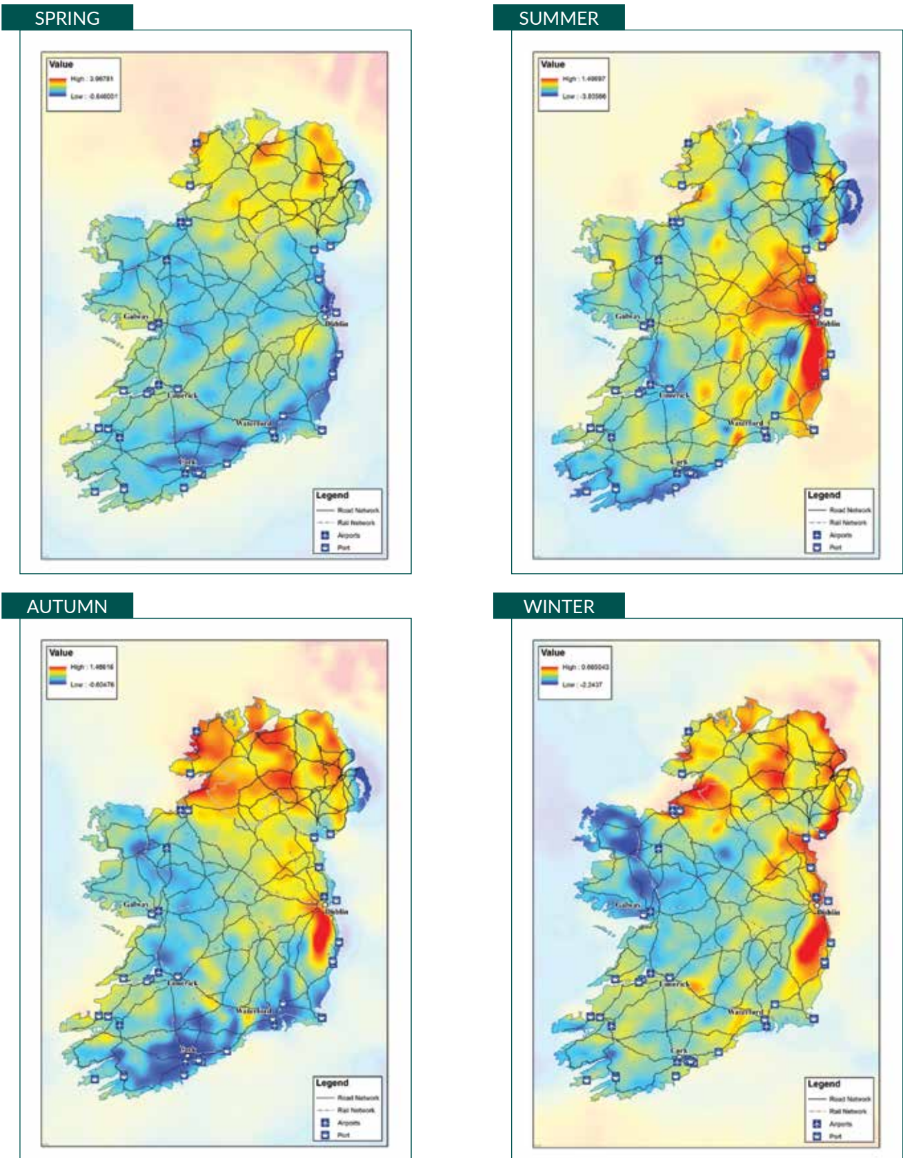
Figure 4.7: Seasonal projected changes (%) in the standard deviation of daily mean 60-m wind speed. (a) Medium- to low-emission ensemble.
