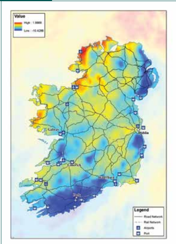
Figure 4.4: Projected changes (%) in seasonal precipitation. (a) medium- to low-emission scenario.
