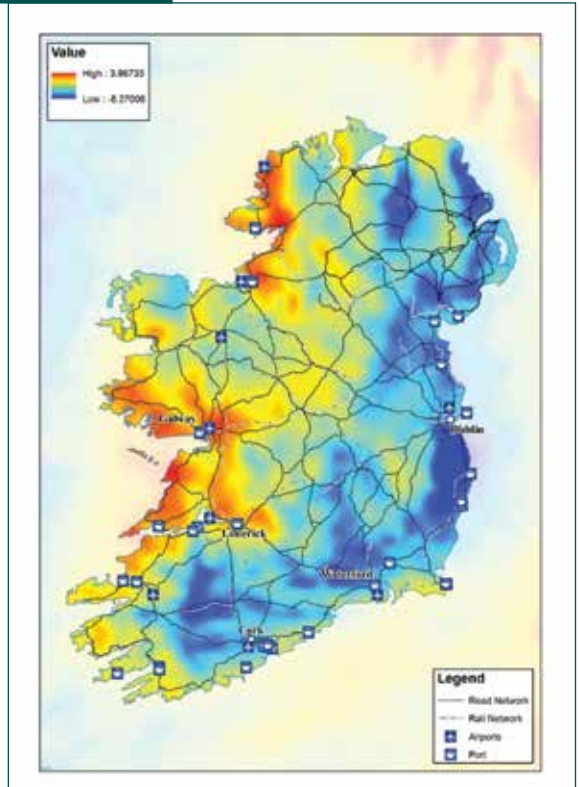
Figure 4.4: Projected changes (%) in seasonal precipitation. (a) medium- to low-emission scenario.
