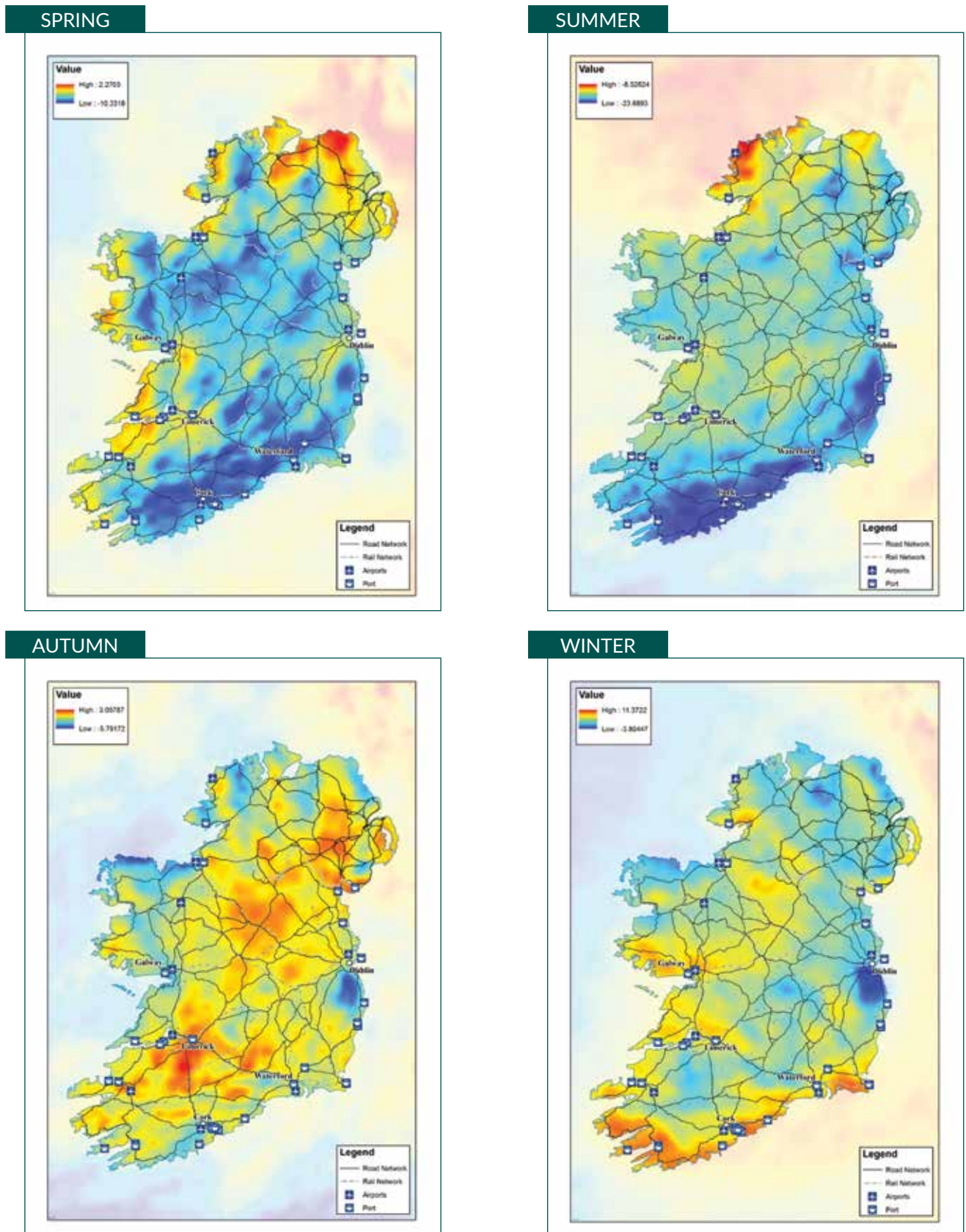
Figure 4.4: Projected changes (%) in seasonal precipitation. (b) high-emission scenario. In each case, the future period 2041–2060 is compared with the past period 1981–2000.
