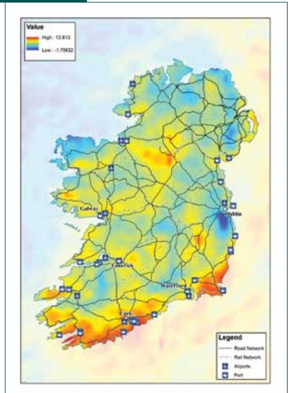
Figure 4.5: Seasonal projected changes (%) in the standard deviation of daily precipitation. (b) high-emission ensemble. In each case, the future period 2041–2060 is compared with the past period 1981–2000.
