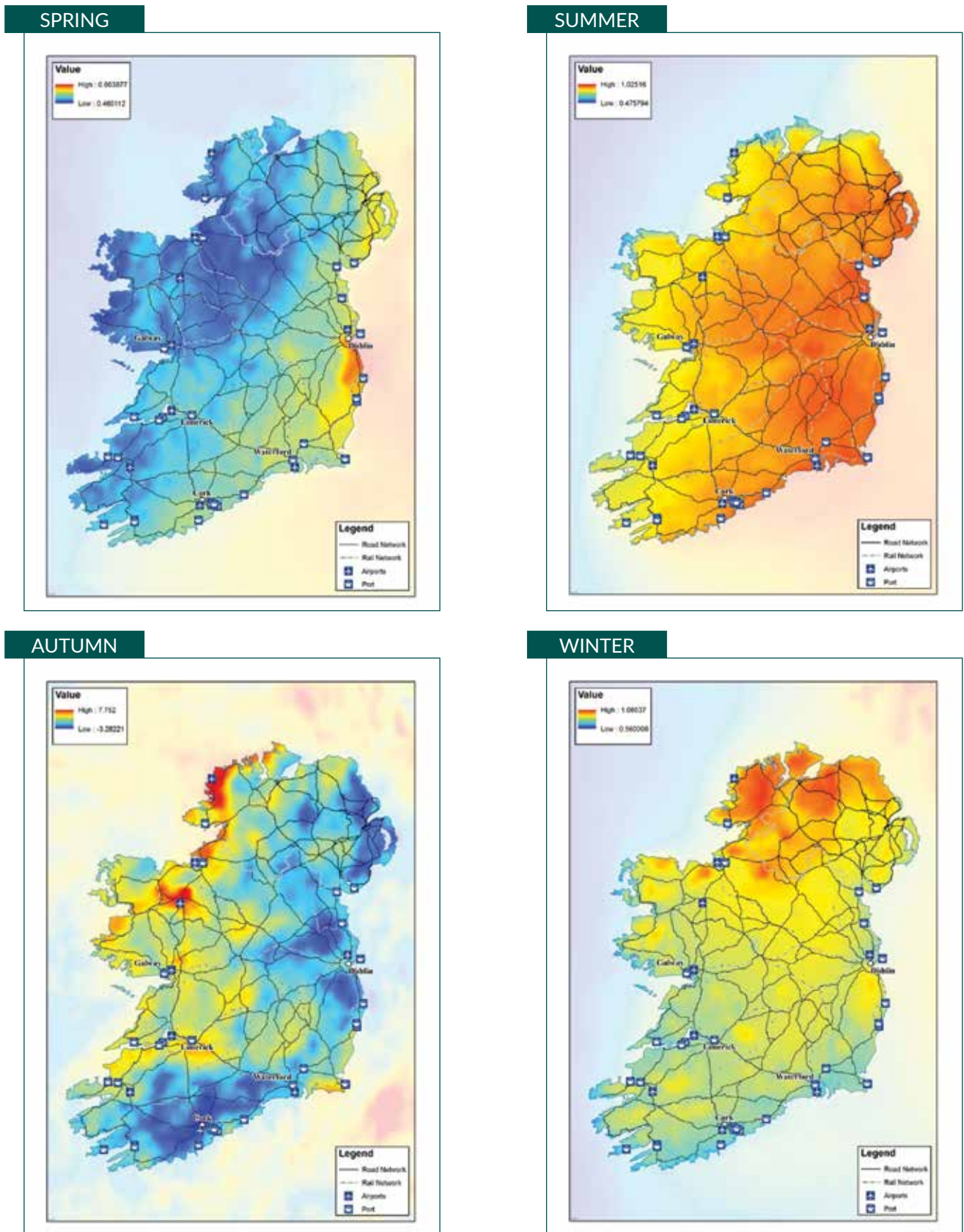
Figure 4.9: The “very likely” seasonal increase in temperature for the (a) medium- to low-emission.
