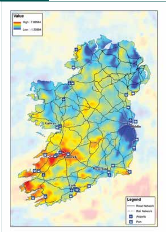
Figure 4.5: Seasonal projected changes (%) in the standard deviation of daily precipitation. (b) high-emission ensemble. In each case, the future period 2041–2060 is compared with the past period 1981–2000.
