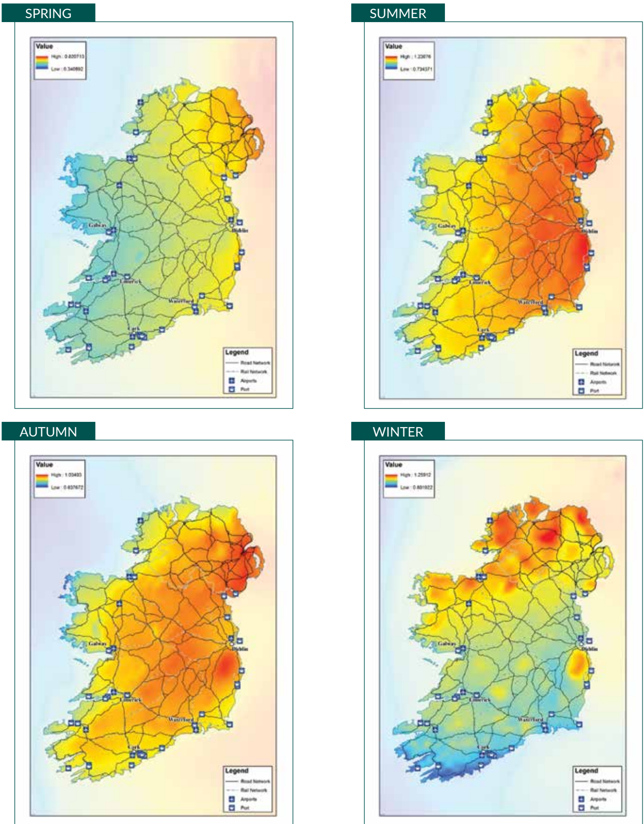
Figure 4.9: The “very likely” seasonal increase in temperature for the (b) high-emission scenarios. In each case, the future period 2041–2060 is compared with the past period 1981–2000.
