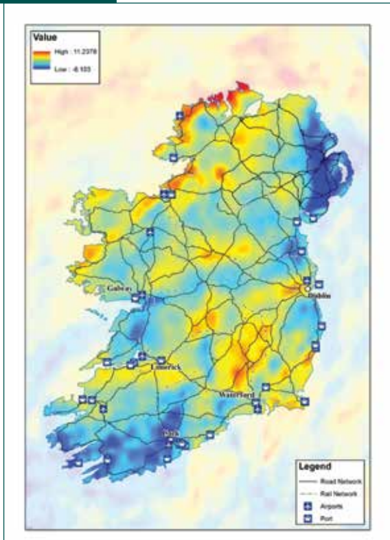
Figure 4.5: Seasonal projected changes (%) in the standard deviation of daily precipitation. (a) medium to low-emission ensemble.
