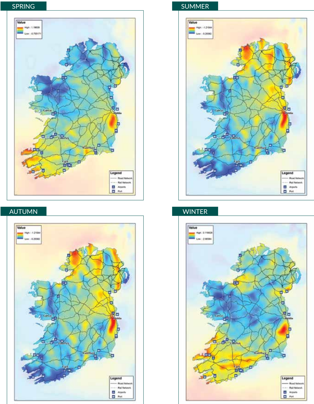
Figure 4.7: Seasonal projected changes (%) in the standard deviation of daily mean 60-m wind speed. (b) high-emission ensemble. In each case, the future period 2041–2060 is compared with the past period 1981–2000.
