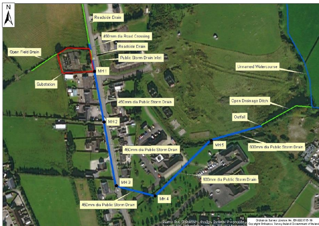
Figure 9 Existing Substation (outlined in red) and public storm drainage network
