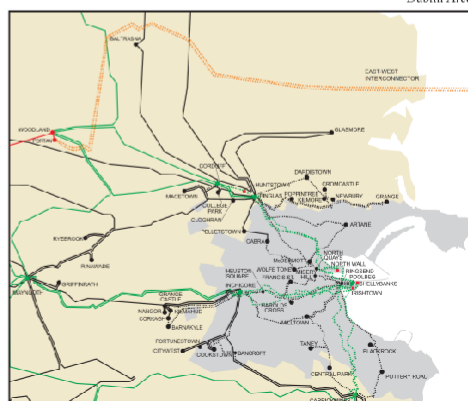
Figure 2 EirGrid Transmission System Map September 2016
