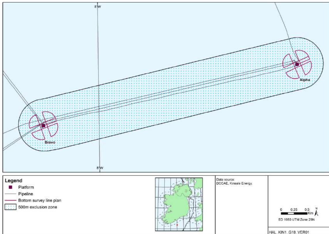
Figure 2.1: Indicative survey lines for KA and KB
