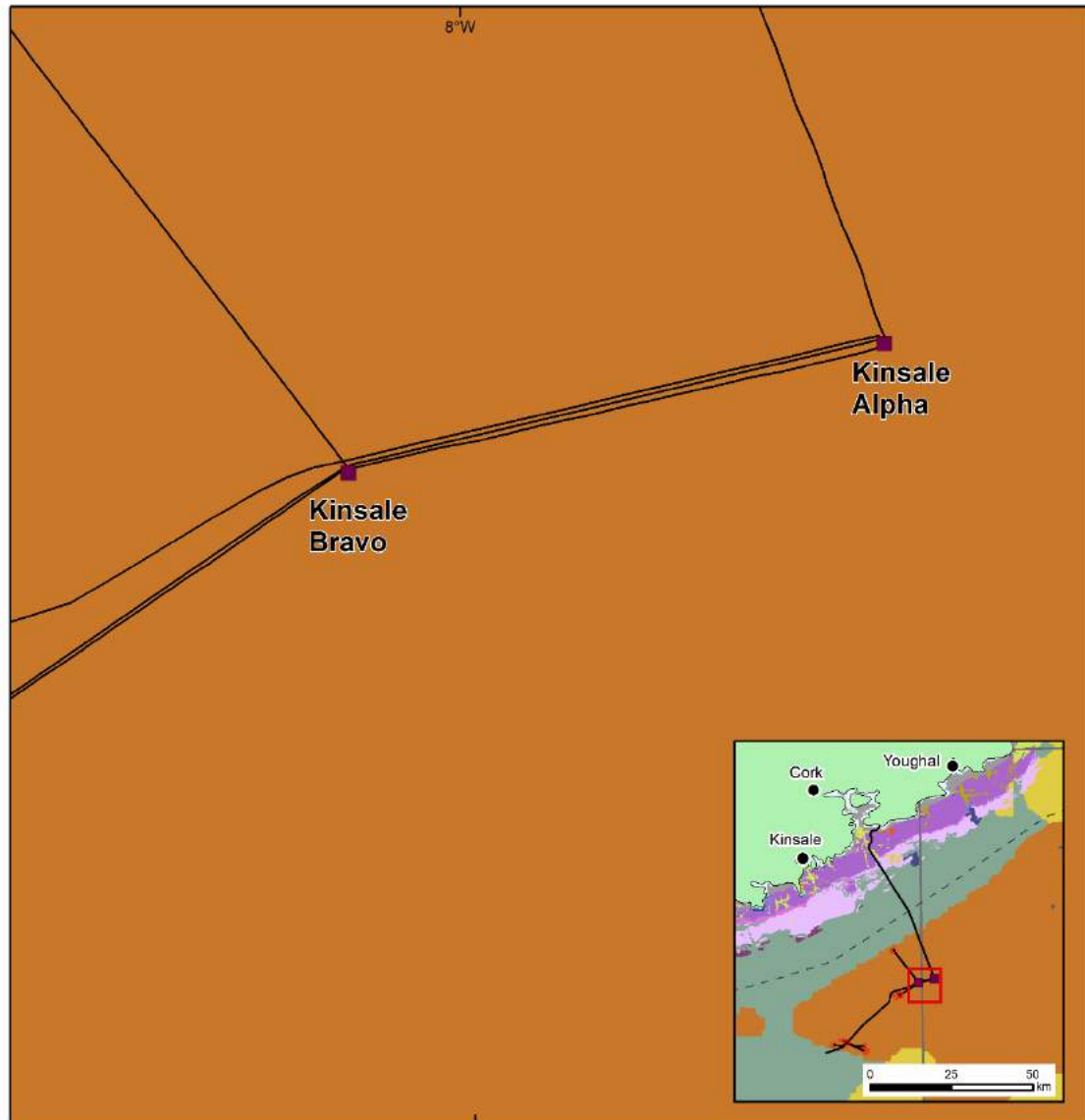
Figure 3.2: Predicted seabed habitats
