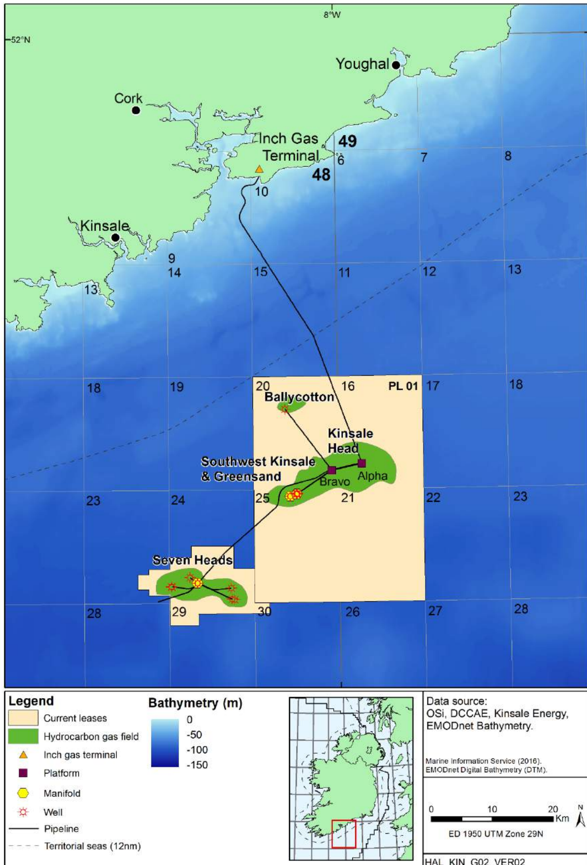
Figure 1.1: Location of the Kinsale Alpha and Bravo platforms in the wider Kinsale Area
