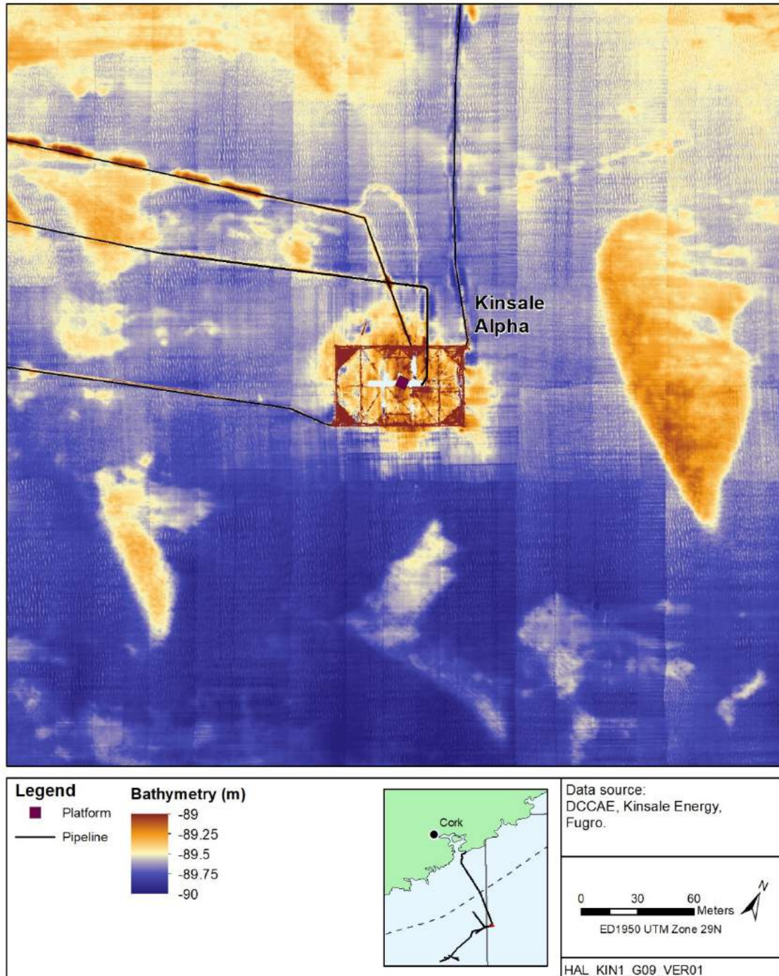
Figure 3.1: Bathymetry a: Kinsale Alpha
